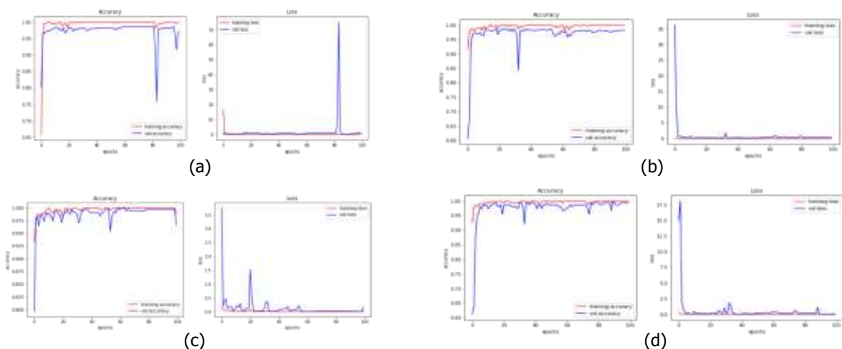
Figure 5. Accuracy and loss graphs of (a) 60:40 scheme, (b) 70:30 scheme, (c) 80:20 scheme, and (d) 90:10 scheme
