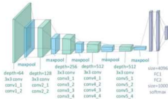
Figure 4. VGG-16 Architecture
